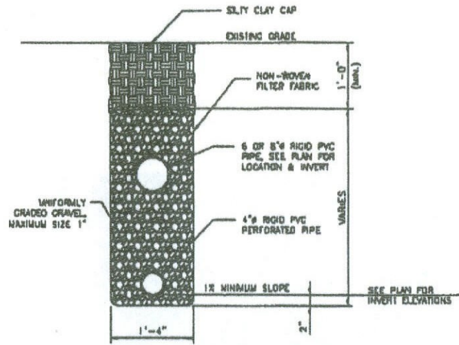
1 B-D DETAIL - SUB-SURFACE DRAIN N.T.S.
